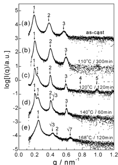
Figure 1. SAXS profiles of through view of the film for SEBS at various thermal histories: (a) as-cast; (b) annealed at 110 ^\circ\text{C} for 300 min; (c) annealed at 120 ^\circ\text{C} for 120 min after annealing at 110 ^\circ\text{C} for 300 min; (d) annealed at 140 ^\circ\text{C} for 60 min after annealing at 110 ^\circ\text{C} for 300 min; and (e) annealed at 168 ^\circ\text{C} for 120 min after annealing at 110 ^\circ\text{C} for 300 min. To avoid overlap, the SAXS profiles were shifted vertically.
